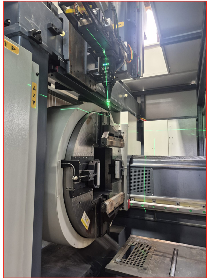
TORCH AND CENTRAL CHUCK
