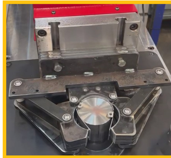
Self-Closing tooling for creating closed shapes (squares, circles etc).
