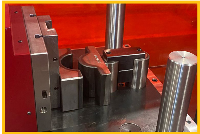
Pipe clamp pressing and forming tool for flat bar bending.
