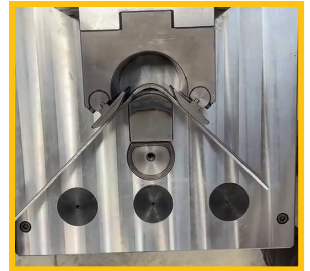
Single die tool, with revolving pin for mark-free bending on plate.
