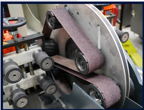
TWIN BELTS
