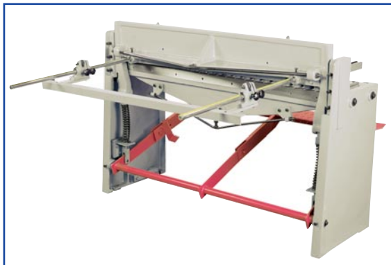
ASTS 1320/1.6 REAR VIEW WITH GUARD REMOVED
