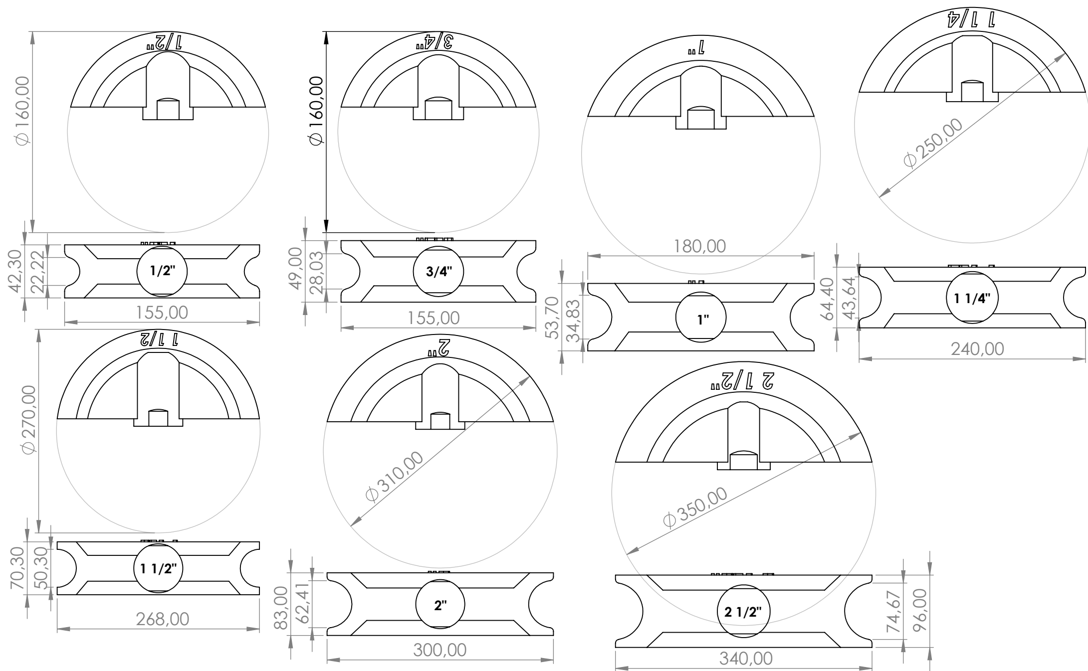
Standard Cast Iron Former Diameters - for pipe bending tool
