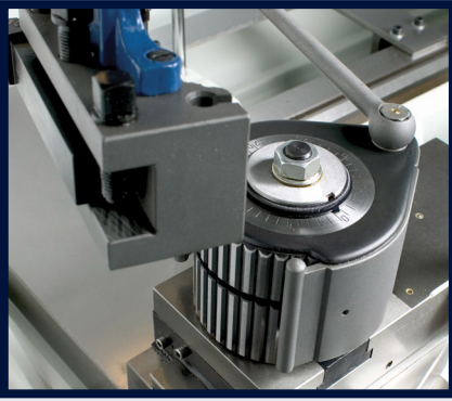
QUICK CHANGE TOOLPOST - OPTIONAL ON SB RANGE, STANDARD ON SG & ST RANGES
